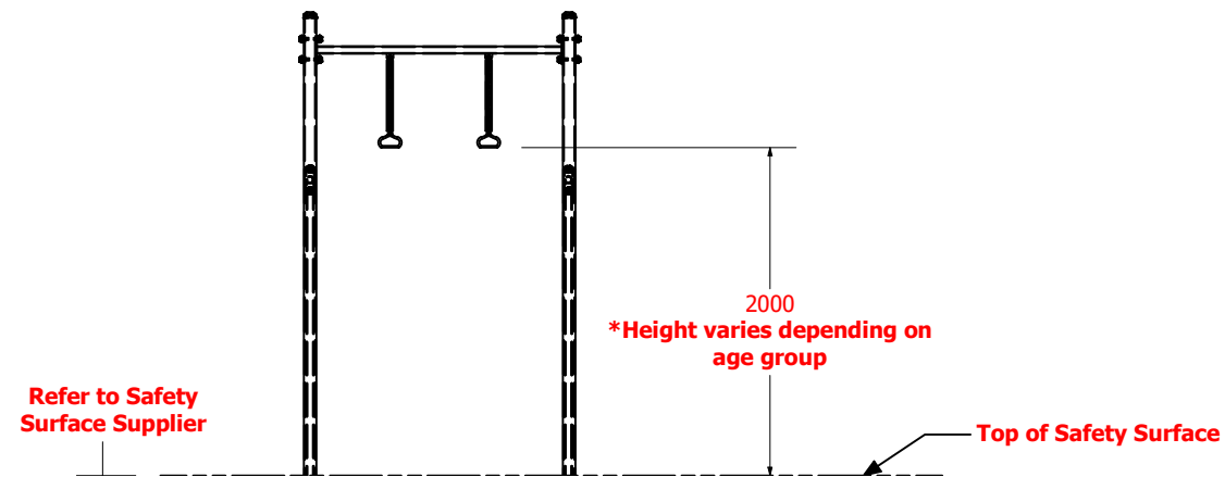
Front Elevation
